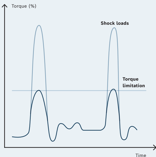
▲ Figure 13: Torque limitation in a Hydraulic Direct Drive.
