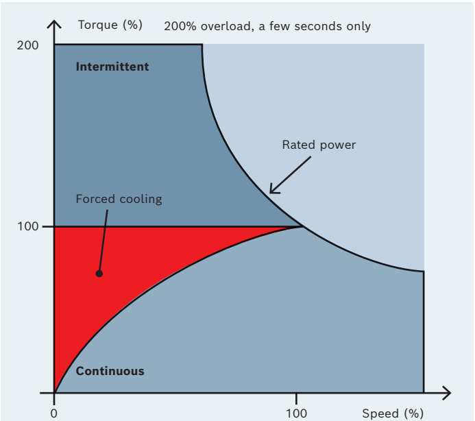
▲ Figure 8: The operating characteristics of a variable-speed DC Drive.
