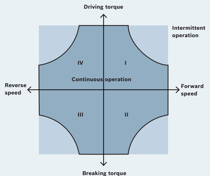
▲ Figure 14: Four-quadrant operation.
