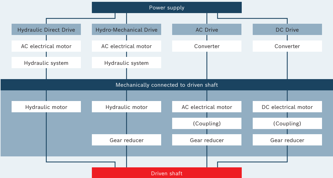
▲ Figure 1: Alternative types of variable-speed drives.
